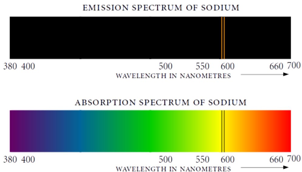
Figure 1.3: Emission (top) and absorption (bottom) spectra of sodium vapour. Sodium emits at its characteristics wavelengths of 589.0 and 589.6 nm. When cold, it absorbs the same wavelengths.
