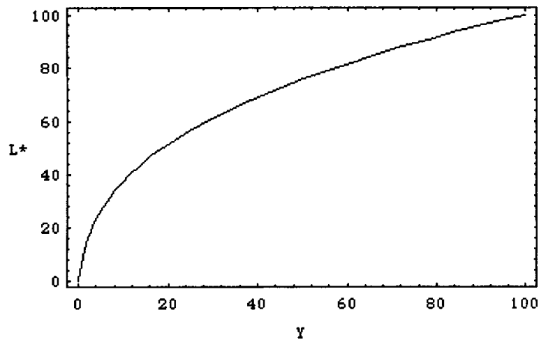
Figure 3.10. L^* -lightness for Y_n = 100 .
