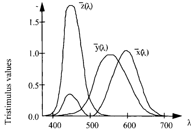
Figure 3.2. The CIE color matching functions \bar{x} , \bar{y} , and \bar{z} for the 2° CIE standard observer.
