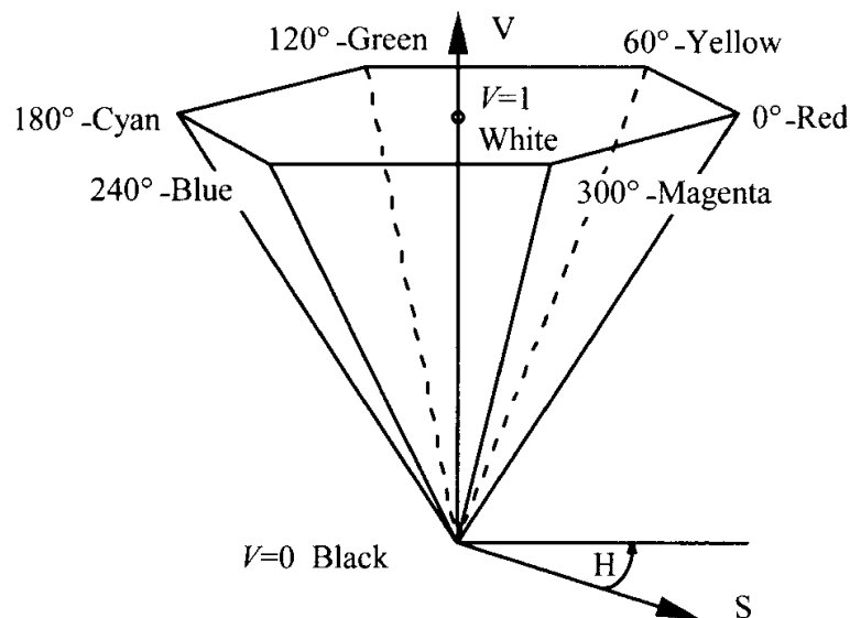
Figure 3.15. Hexacone representation of the HSV color space.
