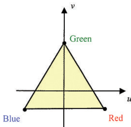
Figure 3.9. The uv -plane of the (YUV)' -model.
